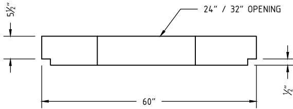
TOP SLAB
