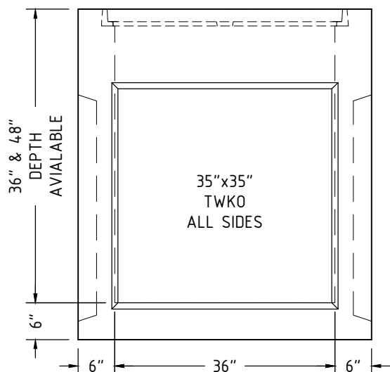
ELEVATION VIEW
