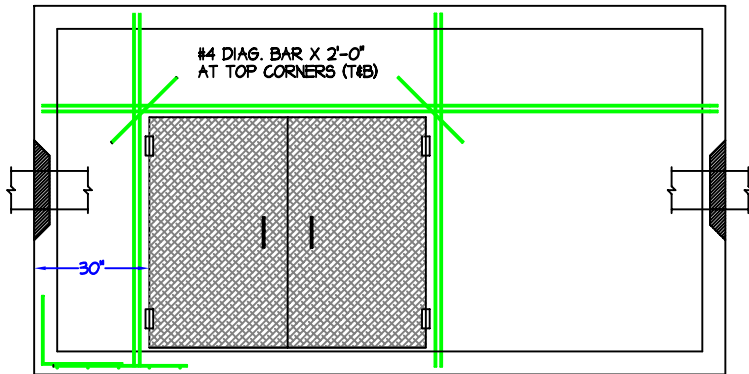
TOP VIEW (LID W/ HATCH)
