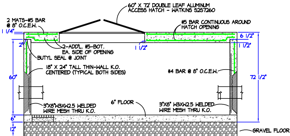
SECTION VIEW
