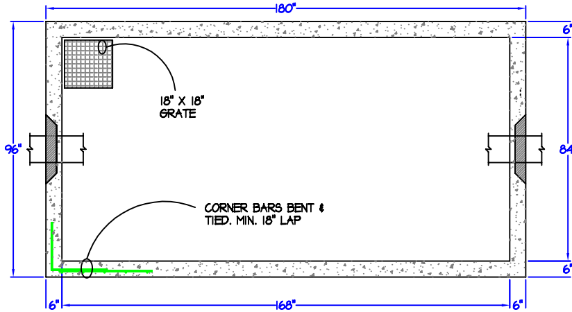
TOP VIEW (FLOOR W/ GRATE)
