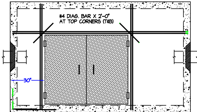
TOP VIEW (LID W/ HATCH)
