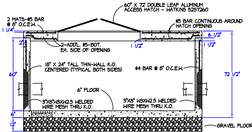
SECTION VIEW
