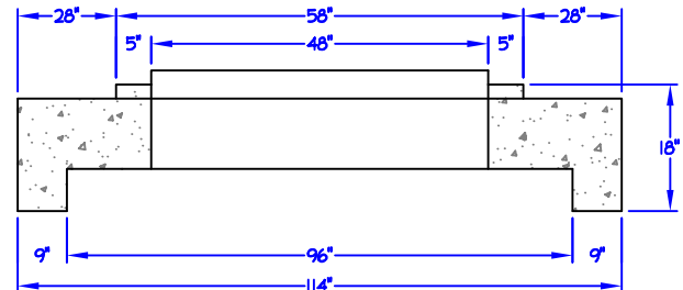
TRANSITION PIECE 96" TO 48"
